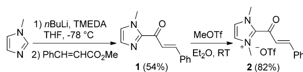
Scheme 3. Synthesis of acyl azolium 2 . TMEDA = tetramethylethylenediamine.
