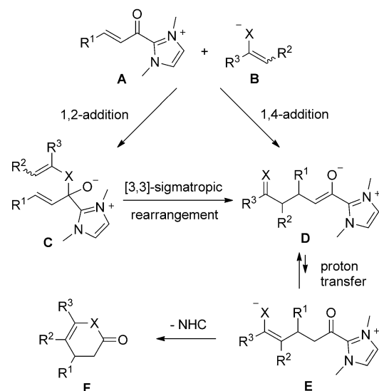
Scheme 2. Possible mechanisms for reaction of enols or enamines with acyl azolium ions A (NHC = N,N' -dimethylimidazoline, X = O, NH).
