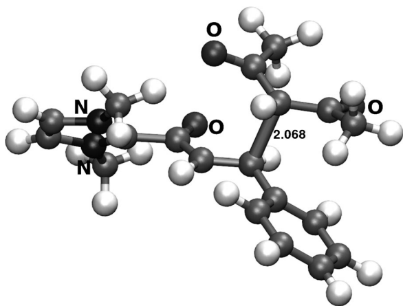
Figure 4. DFT-D3(BJ) + COSMO-optimized transition-state structure for the 1,4-addition of deprotonated acac to acyl azolium 2 . The C–C distance is given in Å.
