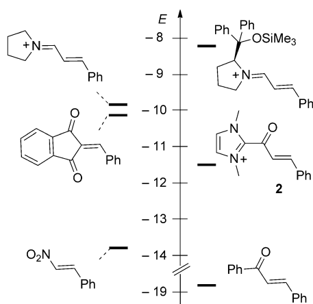
Figure 3. Comparison of electrophilicity parameter E of 2 and other electrophiles. E parameters from Ref. [13]:
