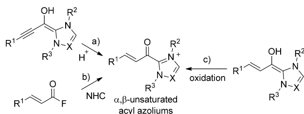
Scheme 1. Different routes for the generation of acyl azolium ions.
