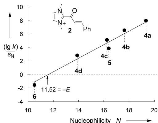
Figure 2. Plot of (\lg k)/s_N versus N for the reactions of 2 with the nucleophiles 4 , 5 , and 6 (solvents are specified in Table 1). Slope of the correlation line is fixed to 1.0 as required by Equation (1).
