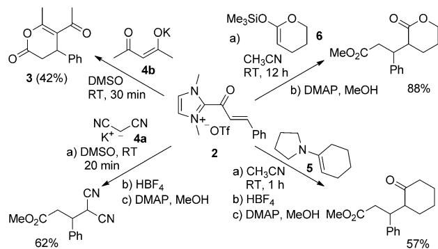
Scheme 4. Reactions of 2 with various nucleophiles. DMSO = dimethyl sulfoxide, 4-DMAP = dimethylaminopyridine.
