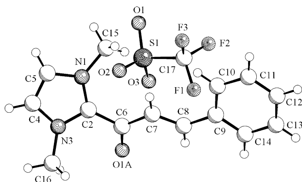
Figure 1. Molecular structure of 2 representing an example of a compound of type A .
